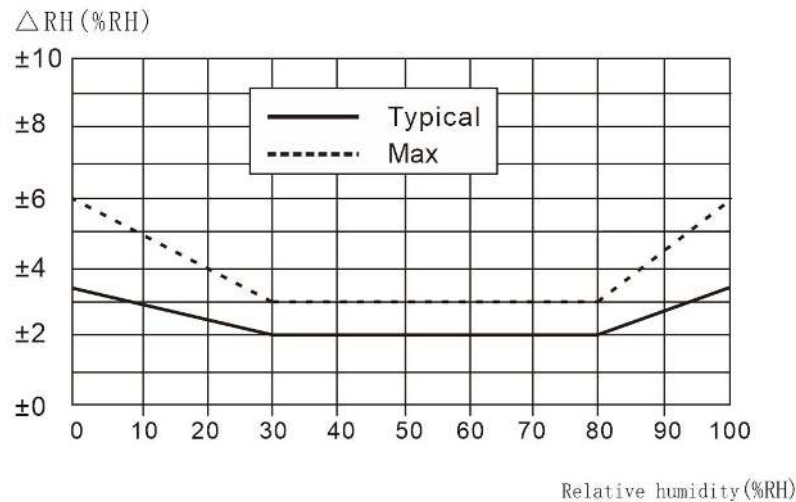
Figure 2. Typical and maximum humidity errors
