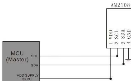
Figure 8. Typical application circuit
