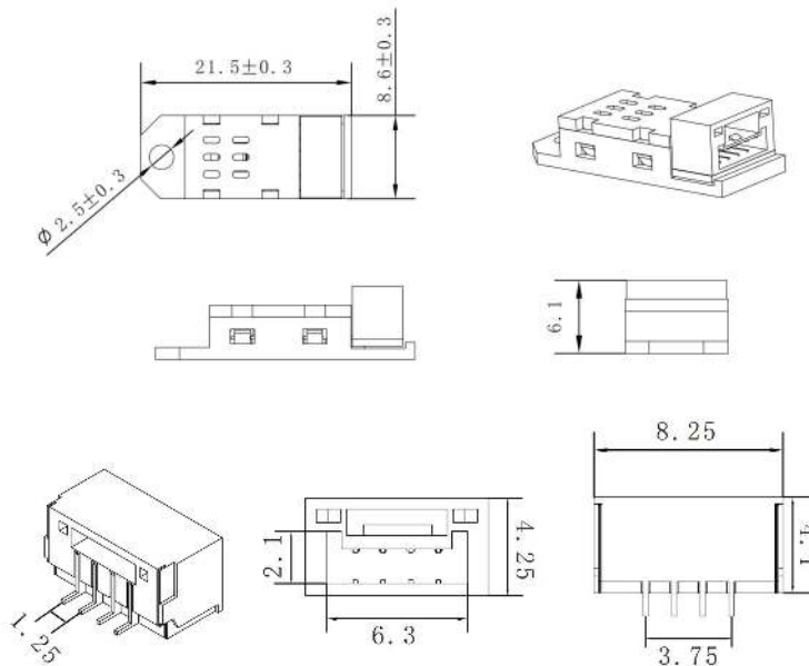
Figure 13. AM2108 sensor encapsulation (unit: mm not specified tolerance: \pm 0.5\text{ mm} )
